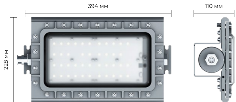
PROEX 40–80 Вт
